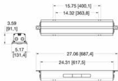
2' Models
