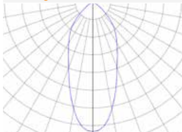
Narrow Pattern
