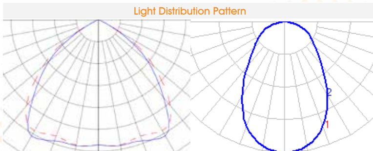
Circular Pattern
