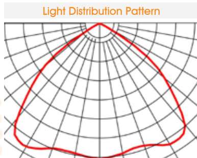
Circular Pattern
