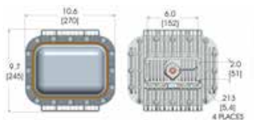
Standard Models
