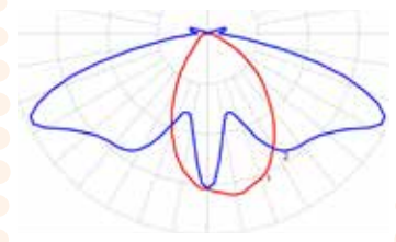
Wide Throw
