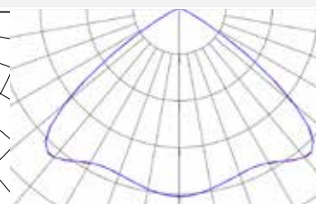
Wide Pattern
