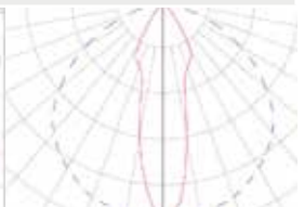
Aisle Pattern
